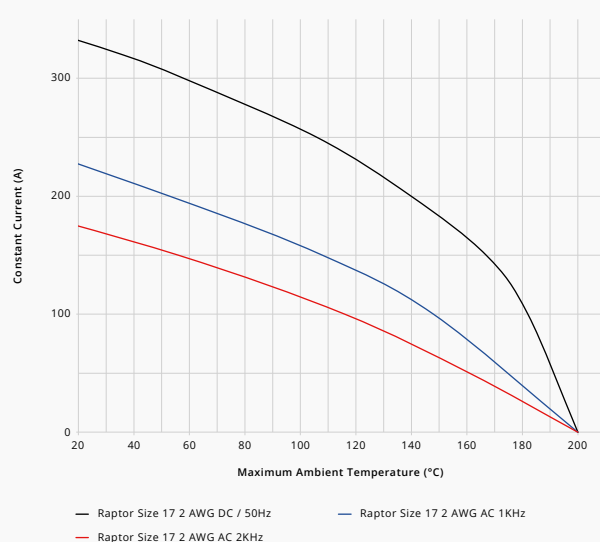
RAPTOR SIZE 17 2 AWG CONSTANT CURRENT AMBIENT TEMPERATURE & FREQUENCY DE-RATING*
