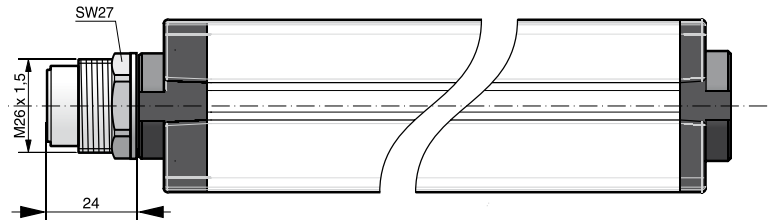
YBB-30...-G026
