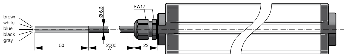
YBB-14...-D020
