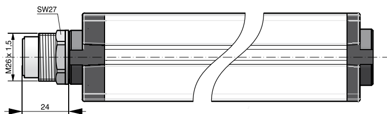
YBB-14...-G026
