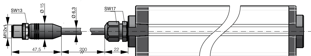
YBB-14...-P012
