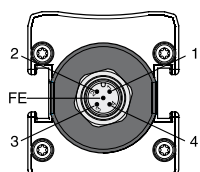
M12 connector
