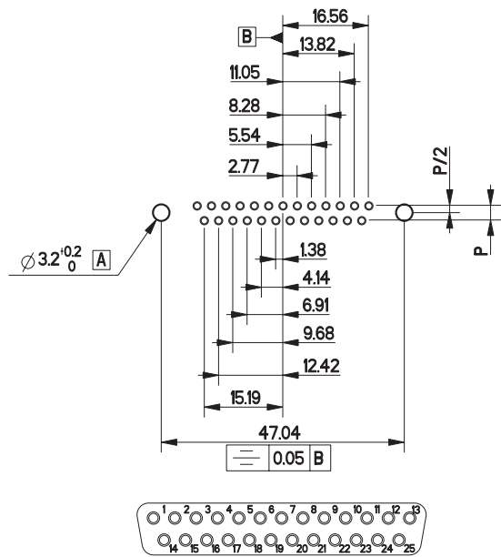
25 Contacts
