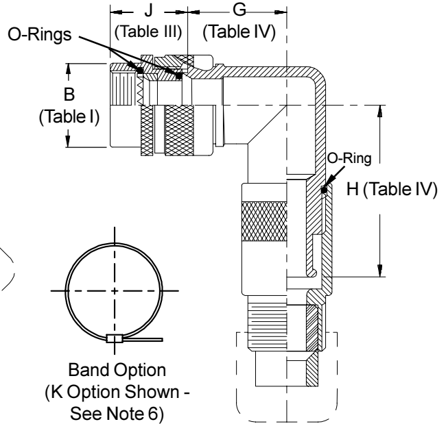
STYLE M Medium Duty (Table XI)
