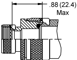
STYLE 2 (STRAIGHT See Note 1)
