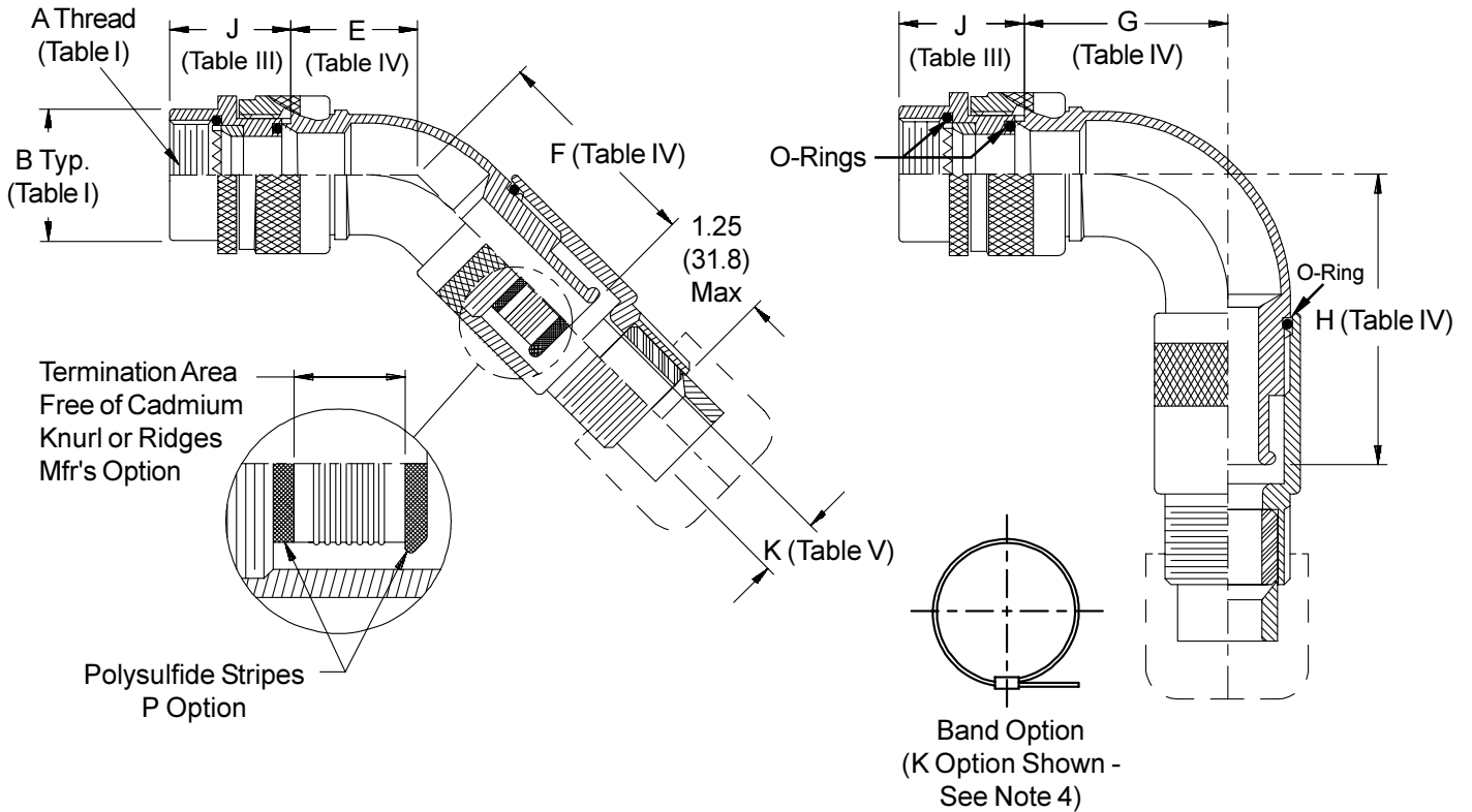
STYLE H Heavy Duty (Table X)
