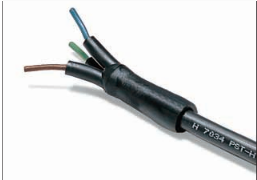
PST-H tubing with a break out boot.
