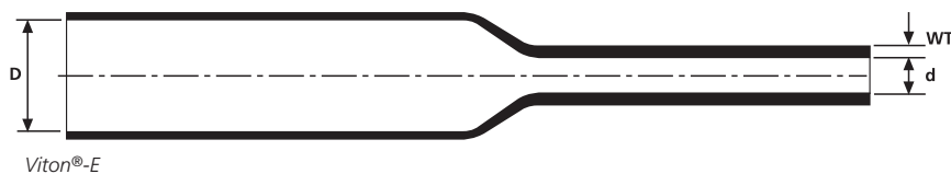
Viton®-E for flexibility and protection against aggressive chemicals.
